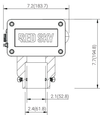
Non-threaded Pole
