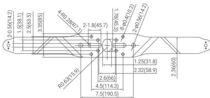
Angled Yoke
