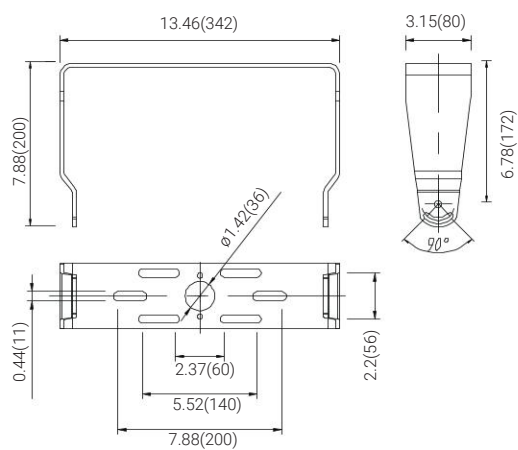
BLK-YOKE
