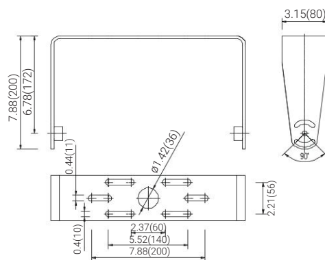
BLK-360Y
