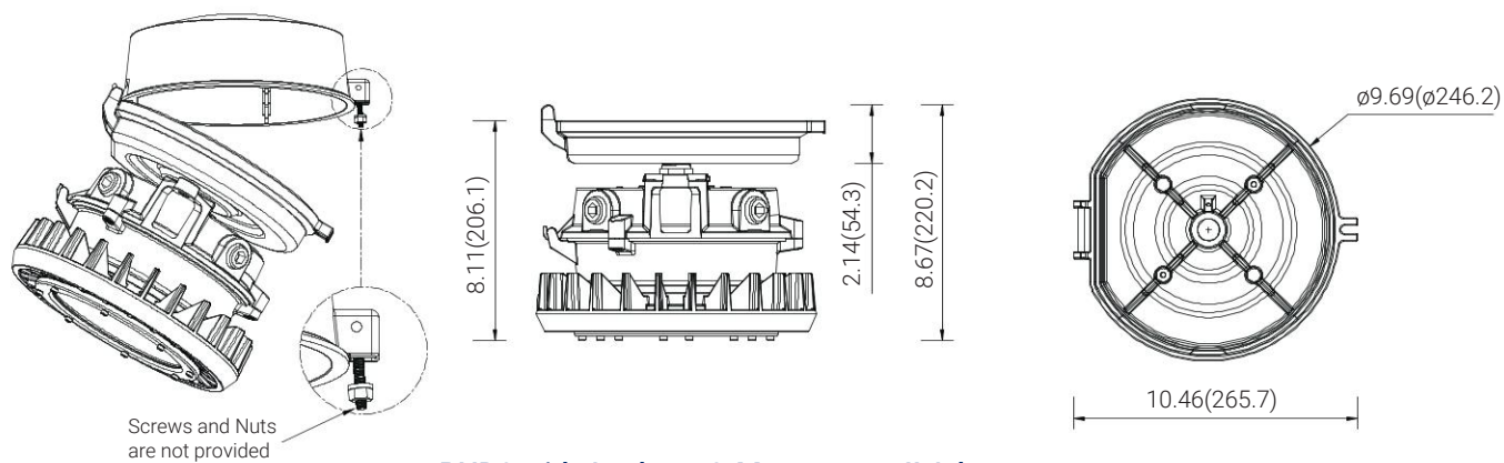
RND2 with Appleton® Mercmaster II Adapter
