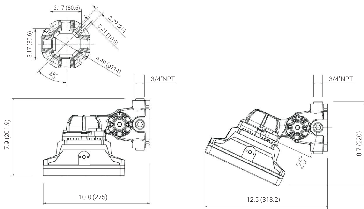
Wall
