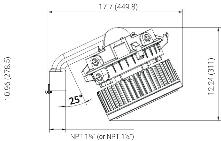
Stanchion
