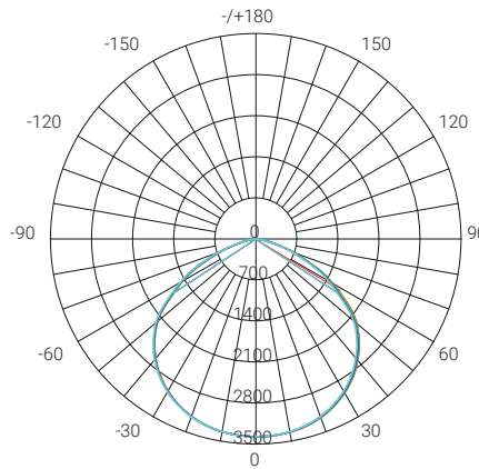
120° NEMA 6 - Wide
