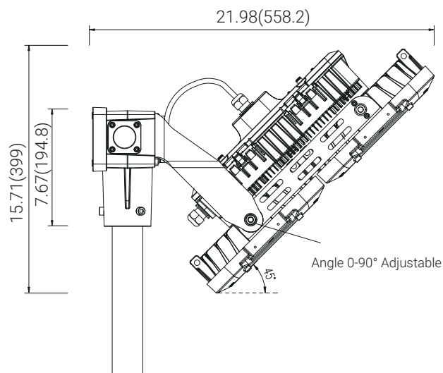
For 50L/60L/70L
