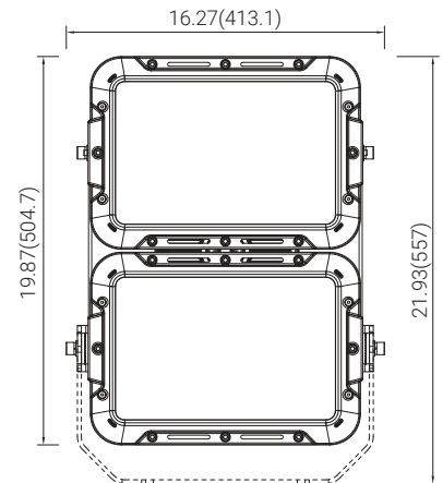
For 50L/60L/70L
