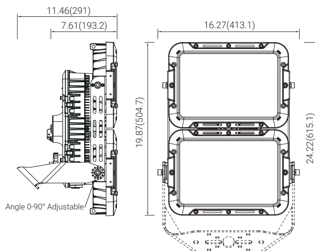
For 50L/60L/70L
