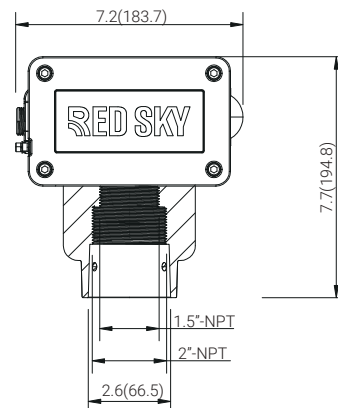
NPT-threaded Pole
