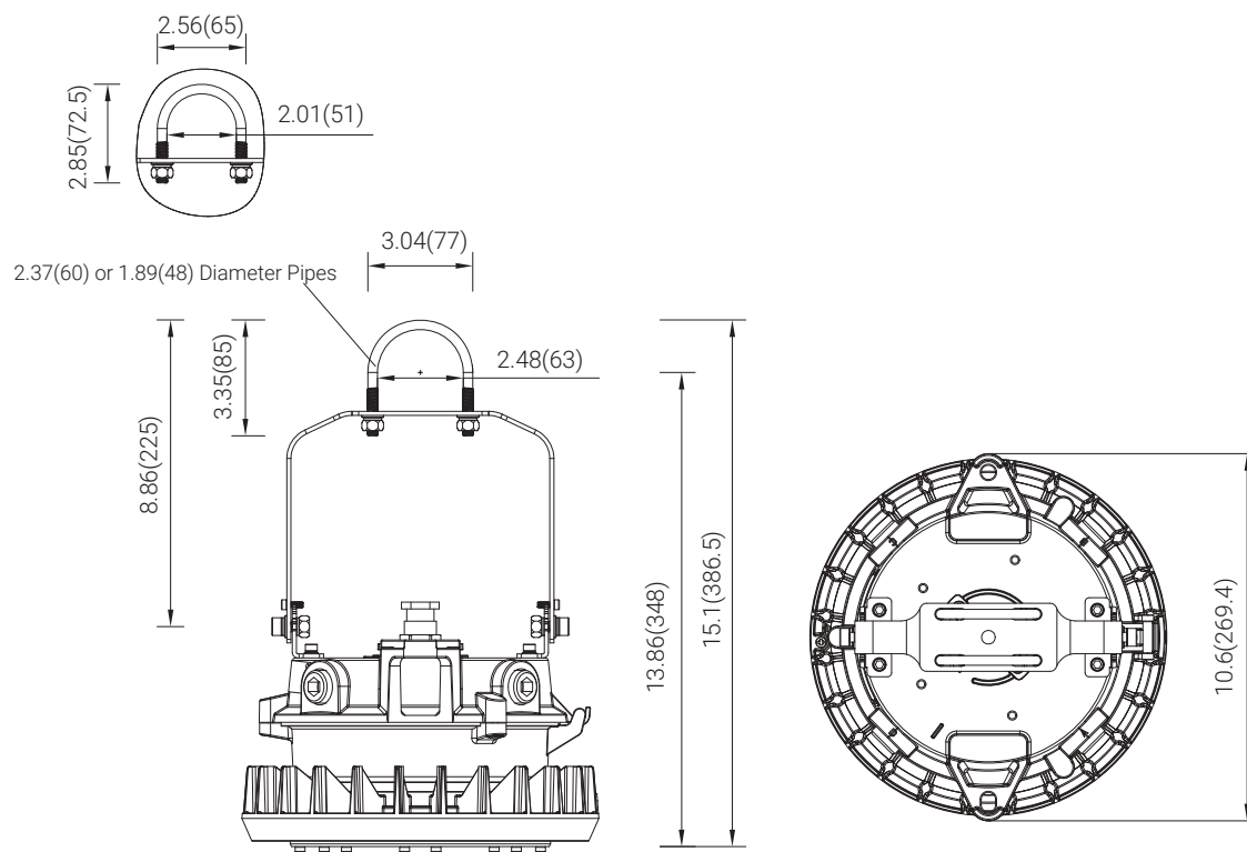
Pole CLAMP01/02
