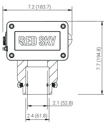
Non-threaded Pole
