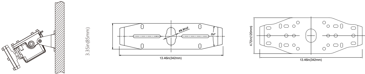
Wall Mount
